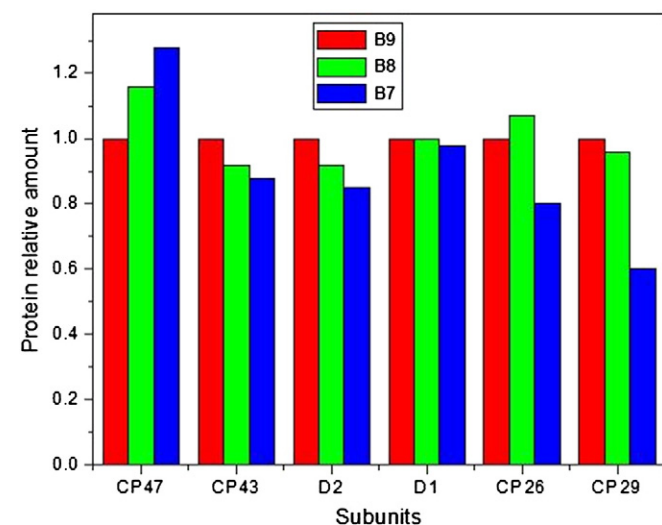
Fig. 5. Protein composition of PSII-LHCII supercomplexes. The number of spectra assigned to individual PSII core subunits and Lhcb monomers (CP26 and CP29) was normalized to the average number of spectra assigned to the core complex polypeptides (calculated as (D1 + D2) / 2 ) in the same fraction. The values are reported relatively to the values determined for each polypeptide in fraction B9.
